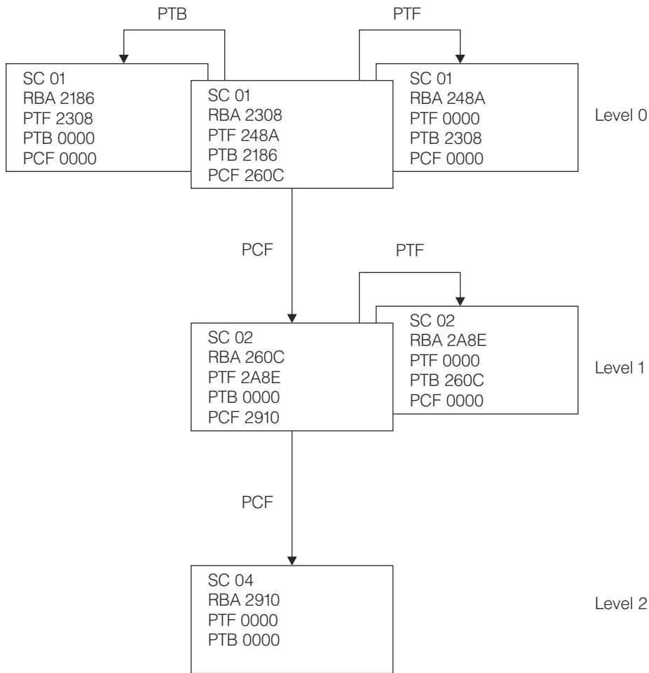
Figure 13. Sample database diagram
