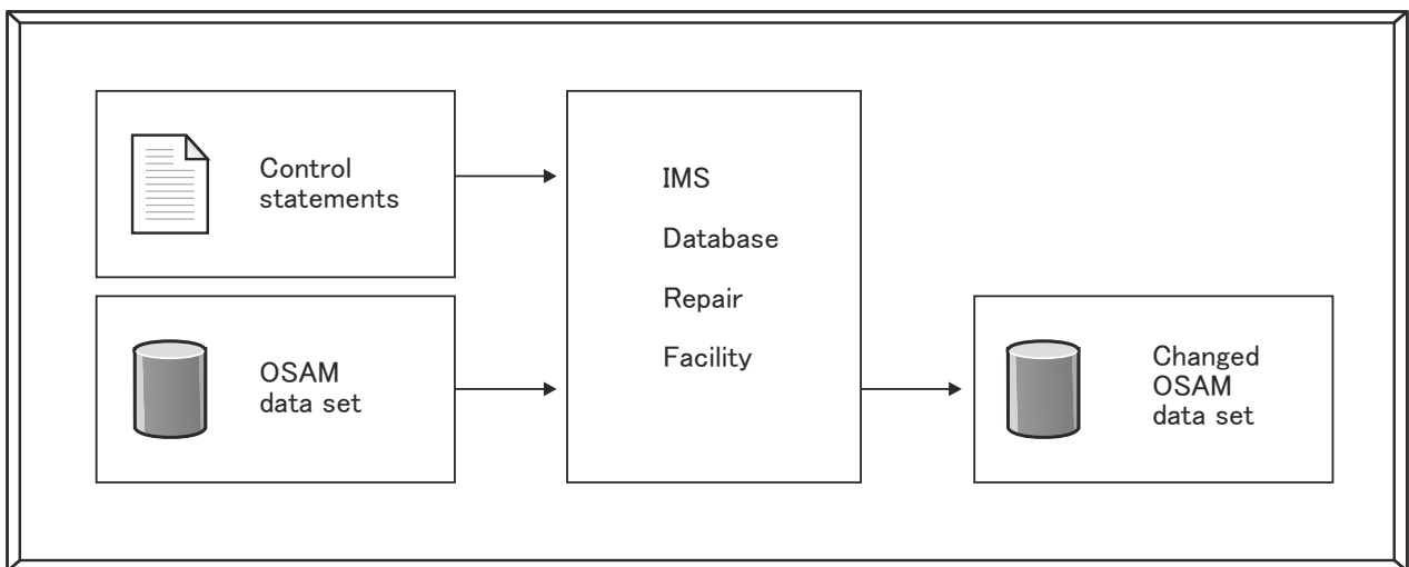
Figure 45. Data flow for batch IMS Database Repair Facility
