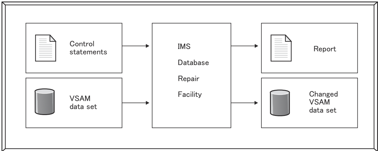
Figure 36. Data flow for batch IMS Database Repair Facility
